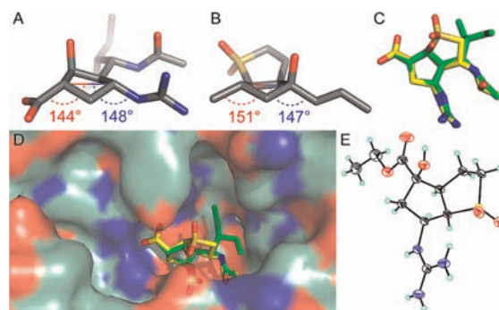
Figure 2. X-ray structural data and in silico docking results. (A) Structure of peramivir bound in the enzyme active site (from PDB 2HTU); (B) structure of 5a (CCDC 766248); (C) overlay of enzyme-bound peramivir (green) with the docked structure of 15 (yellow; calculated in MOLOC); (D) peramivir and 15 pictured inside the neuraminidase active site; (E) small-molecule X-ray structure of the ethyl ester hydrochloride of 10 .
